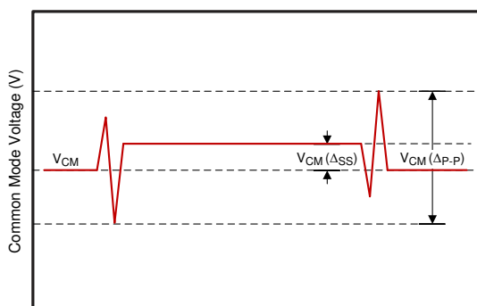
图 6-1. Common Mode Voltage
