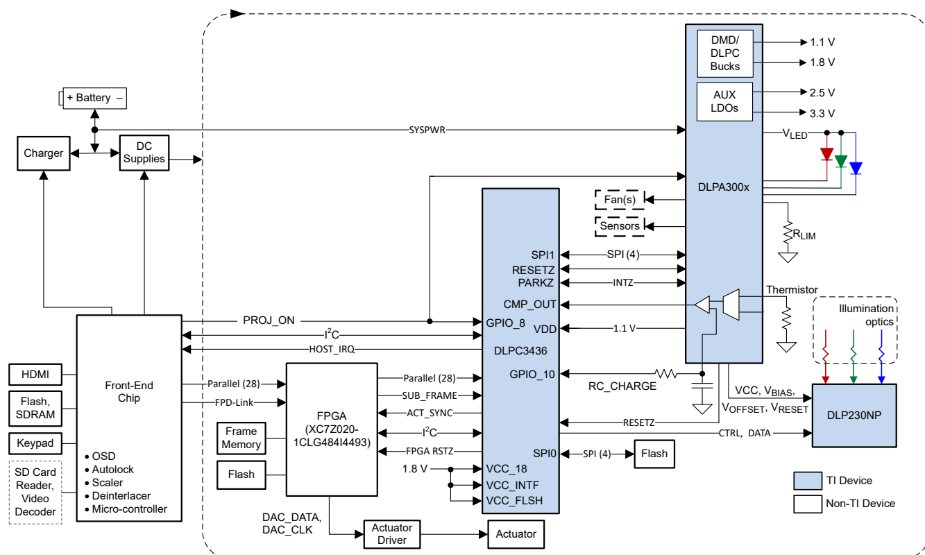
图 8-2. Typical Application Diagram (using DLPA300x)
