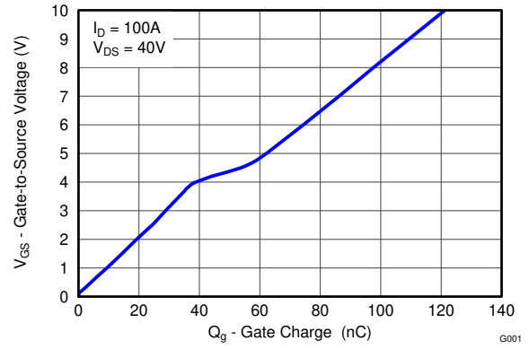
栅极电荷
