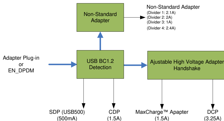
图 8-1. USB D+/D- Detection
