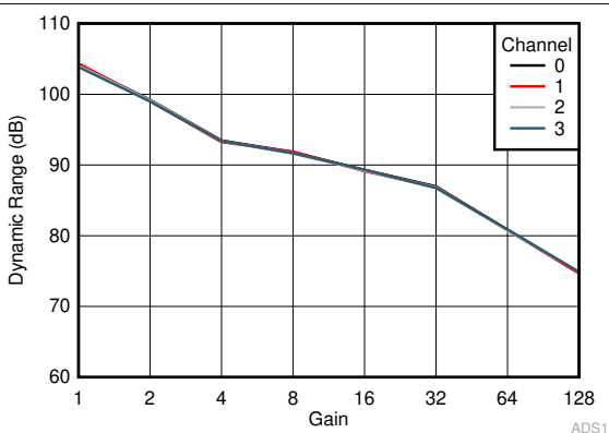
图 6-22. Dynamic Range vs Gain
