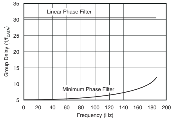
图 7-18. FIR Group Delay ( f_{DATA} = 500SPS )
