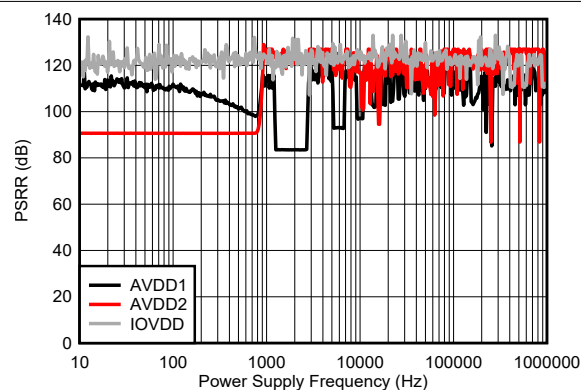
图 5-34. PSRR vs Power-Supply Frequency
