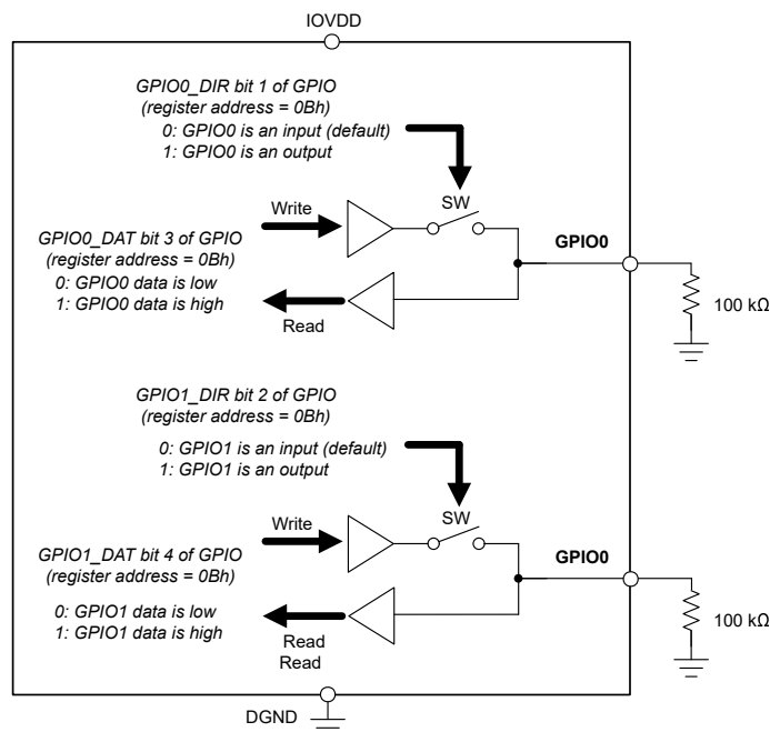
图 7-19. GPIO Operation
