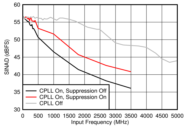
图 7-42. SINAD vs F_{IN} and C-PLL modes
