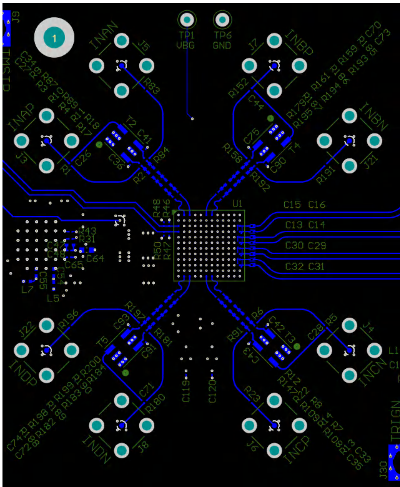
图 9-5. Top Layer Routing: Analog Inputs (INA±, INB±, INC±, IND±), TMSTP± and D[3:0]± Routing
