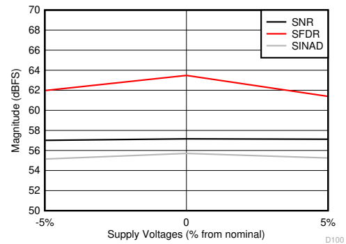
图 7-60. SNR, SFDR and SINAD vs Supply Voltage
