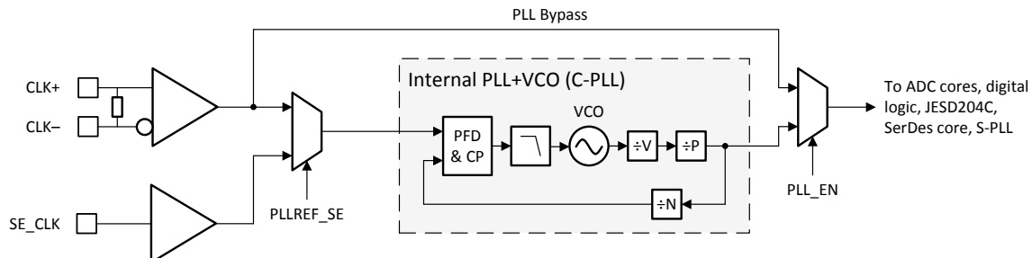
图 8-4. Converter PLL (C-PLL) Architecture
