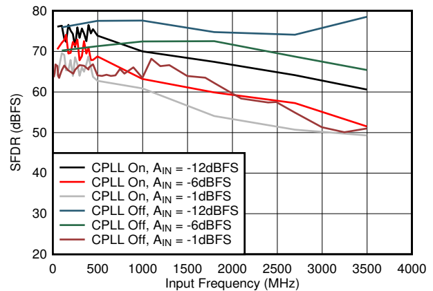
图 7-48. SFDR vs A_{IN} and C-PLL
