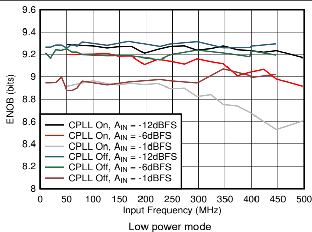
图 7-57. ENOB vs A_{IN} and C-PLL
