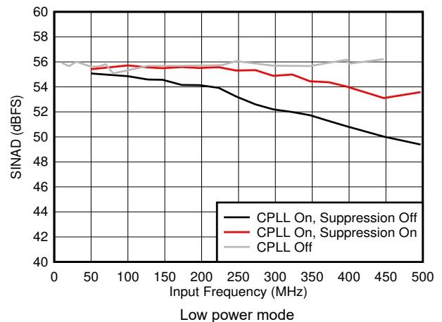
图 7-46. SINAD vs F_{IN} and C-PLL modes
