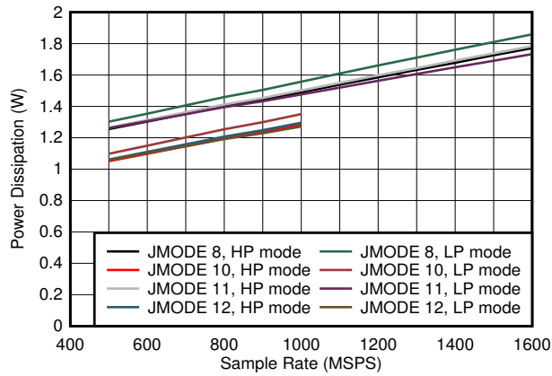
图 8-91. Dual Channel, Power Dissipation vs F_S and JMODE 8 - 12
