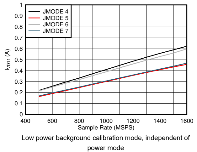
图 8-86. Quad Channel, I_{VD11} vs F_S and JMODE 4 - 7
