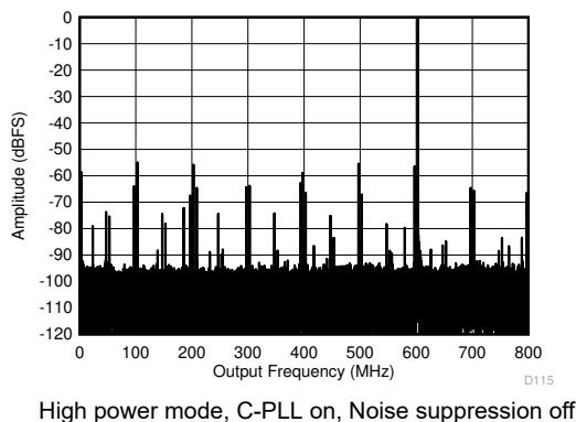
图 8-9. Single Tone FFT at 997 MHz and -1 dBFS
