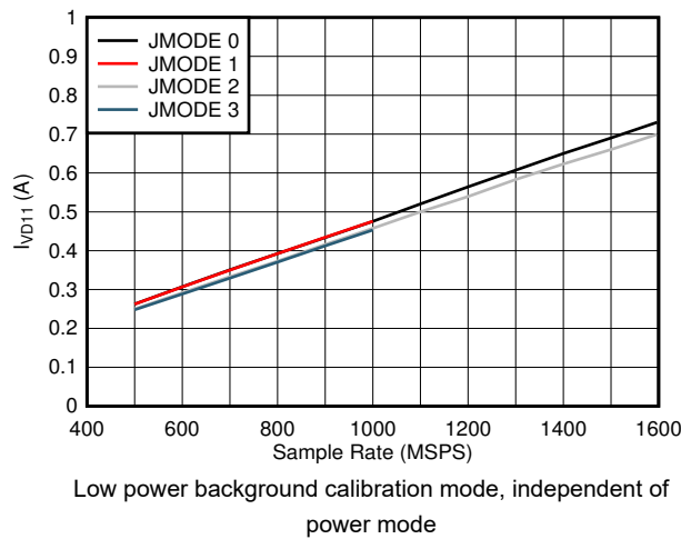
图 8-85. Quad Channel, I_{VD11} vs F_S and JMODE 0 - 3
