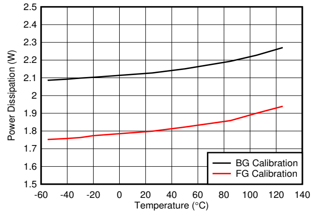
图 8-122. Dual Channel, Power Dissipation vs Temperature
