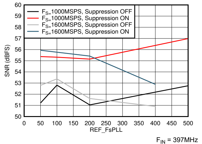
图 8-38. SNR vs F_{REF} and Suppression
