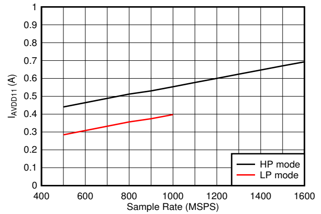
图 8-84. Quad Channel, I_{VA11} vs F_S
