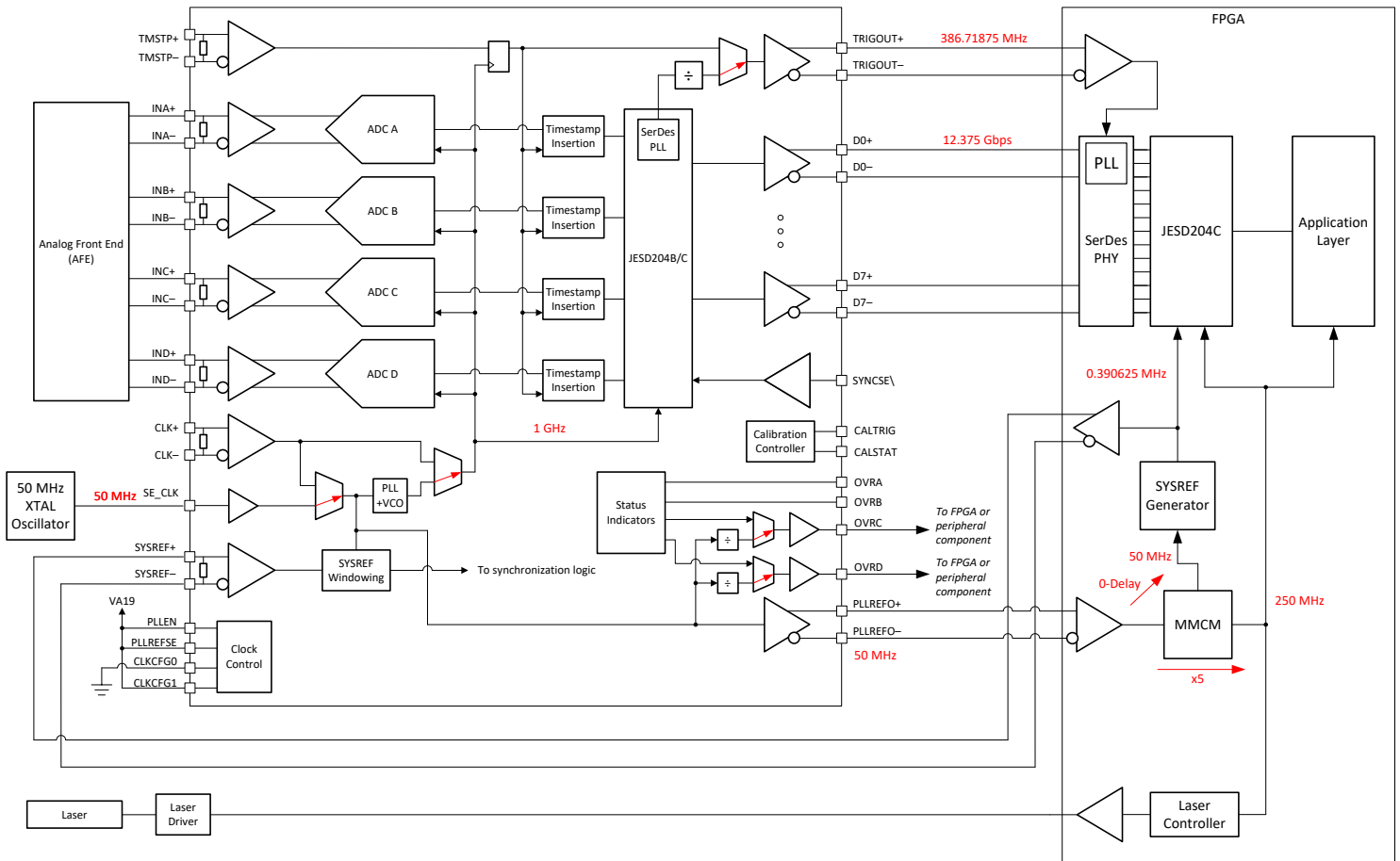
图 10-1. Typical Configuration for a LiDAR Digitizer
