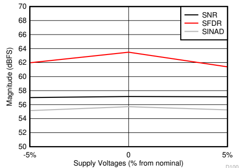
图 8-60. SNR, SFDR and SINAD vs Supply Voltage
