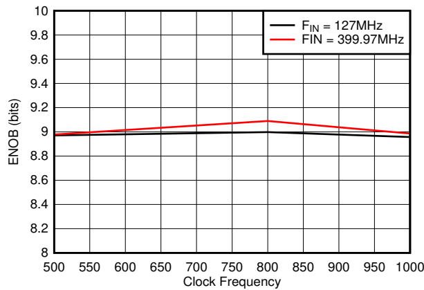
图 8-31. ENOB vs Sample Rate
