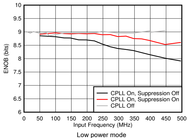
图 8-47. ENOB vs F_{IN} and C-PLL modes
