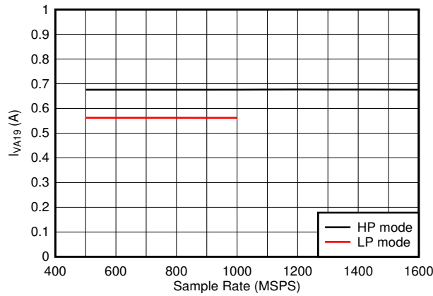
图 8-83. Quad Channel, I_{VA19} vs F_S
