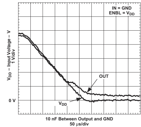
图 7-20. Output Behavior vs V_{DD} (UCC37321)
