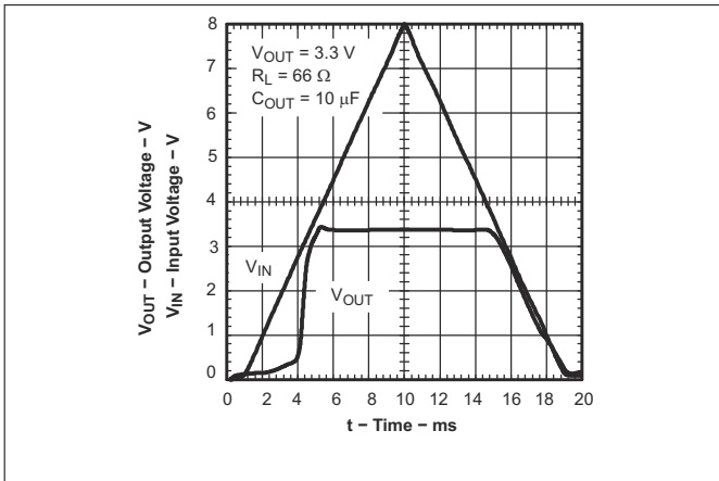
图 8-4. Power-Up and Power-Down for Legacy Chip
