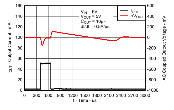
图 8-9. Load Transient Response for New Chip
