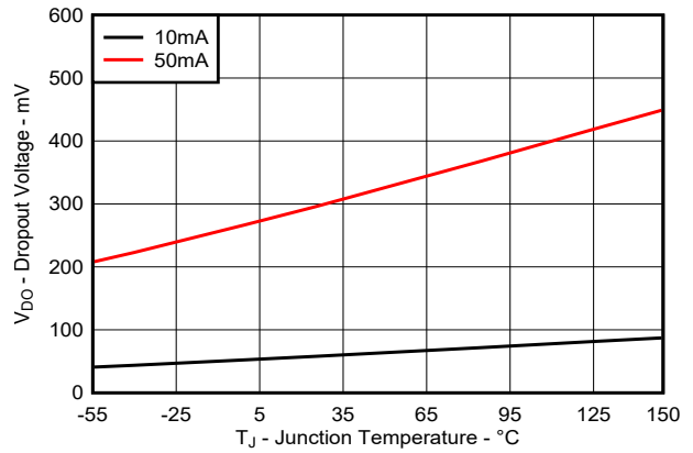
图 6-14. Dropout Voltage vs Junction Temperature for New Chip
