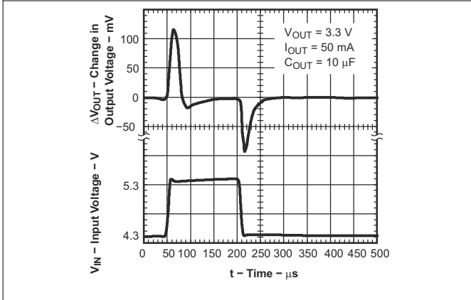
图 8-6. Line Transient Response for Legacy Chip
