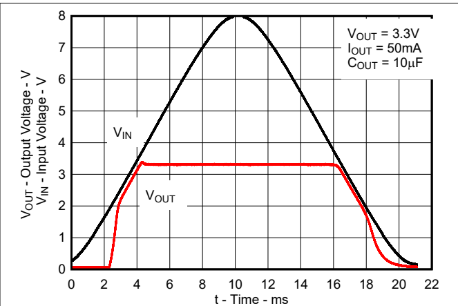
图 8-5. Power-Up and Power-Down for New Chip
