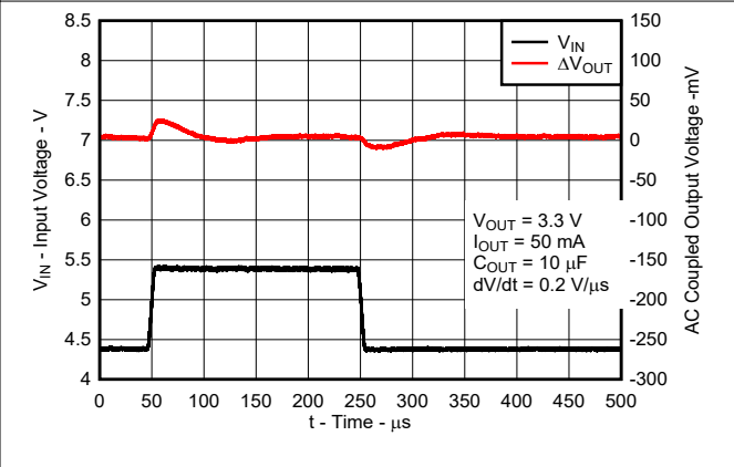
图 8-7. Line Transient Response for New Chip
