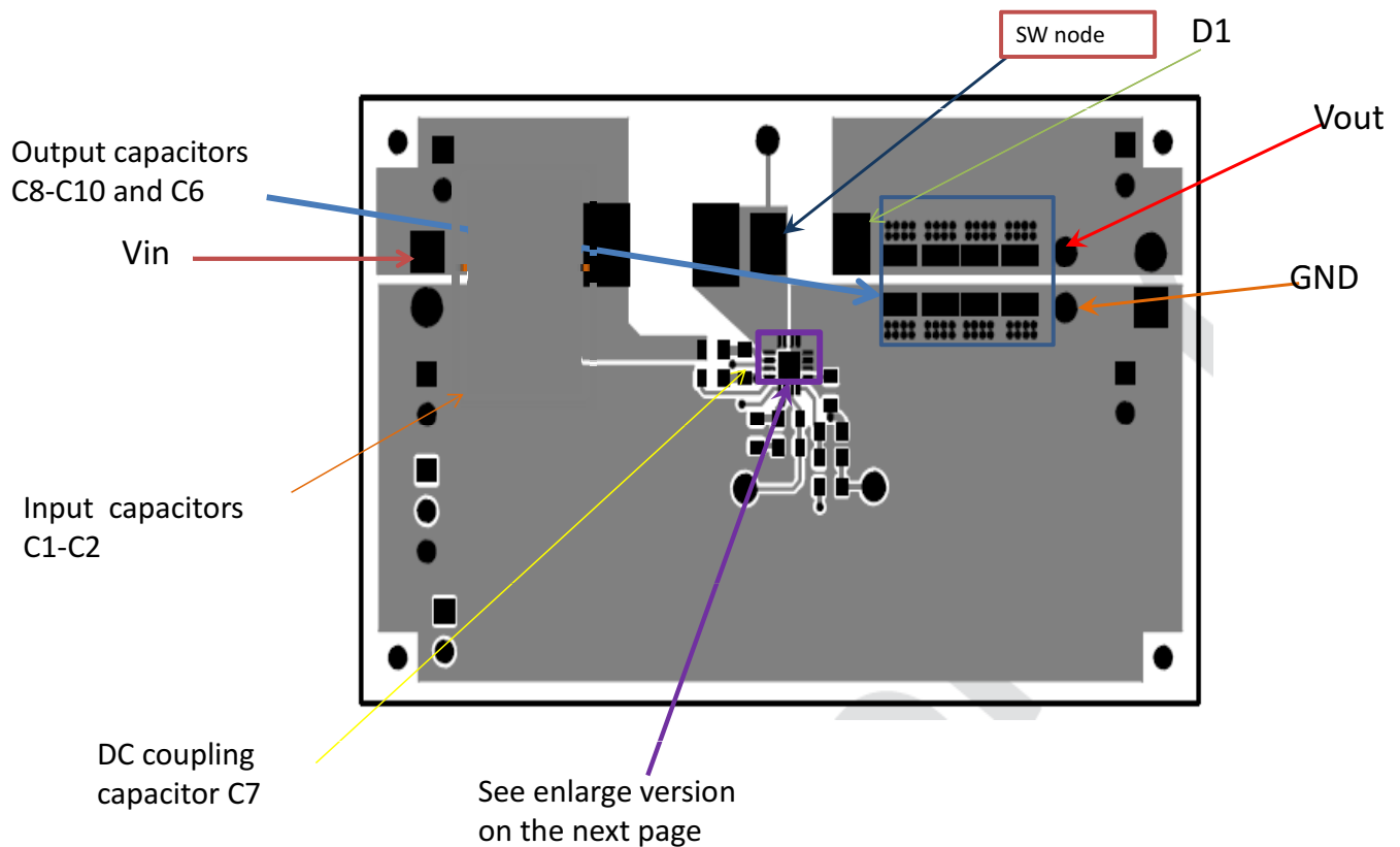
图 11-1. TPS55340 Top-Side Layout
