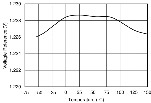
图 7-3. Feedback Voltage Reference vs Temperature
