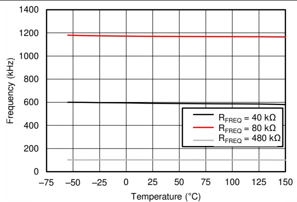
图 7-6. Frequency vs Temperature
