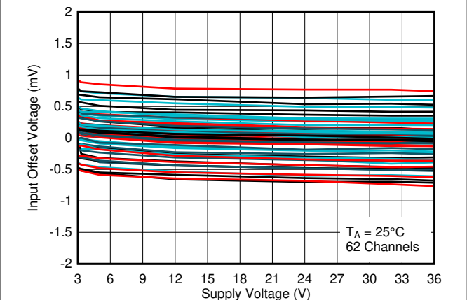
图 7-12. Input Offset Voltage vs. Supply Voltage at 25^\circ\text{C}
