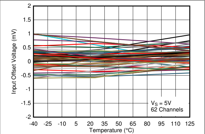
图 7-8. Input Offset Voltage vs. Temperature at 5V
