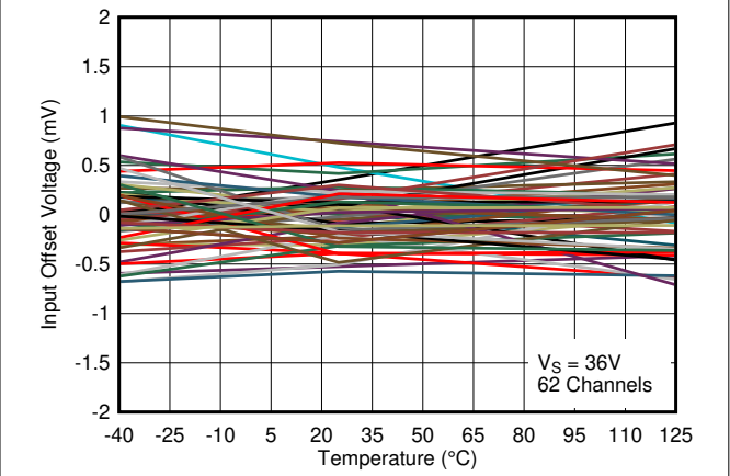
图 7-10. Input Offset Voltage vs. Temperature at 36V
