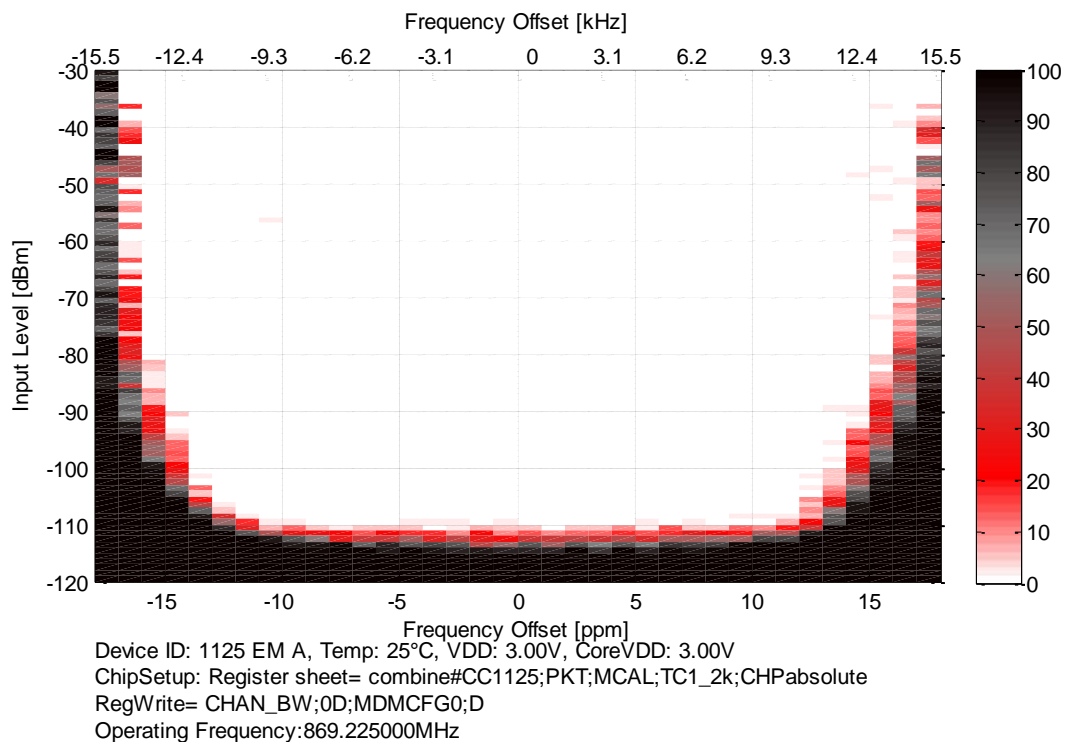
Figure 6. “Bathtub Plot”. 1.2 kbit/s, \pm 1.2 kHz, 19.2 kHz Filter Bandwidth with FB2PLL
