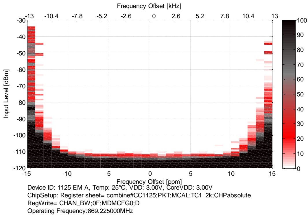
Figure 5. “Bathtub Plot”. 1.2 kbit/s, \pm 1.2 kHz, 16.6 kHz Filter Bandwidth with FB2PLL
