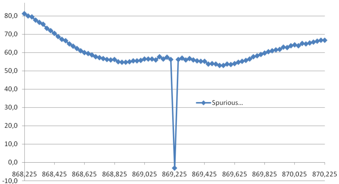
Figure 8. Spurious Response Rejection @1.2 kbit/s, 19.2 kHz Filter Bandwidth with FB2PLL
