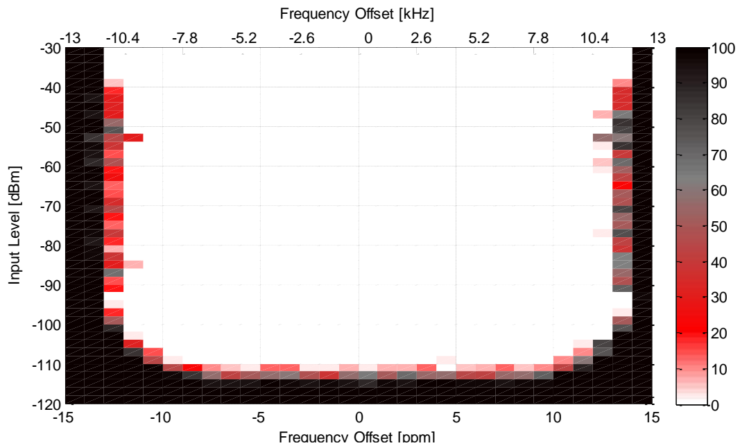
Figure 1. FB2PLL Enabled, 4 byte Preamble (4.8 kbit/s, 16.6 kHz Filter Bandwidth)
