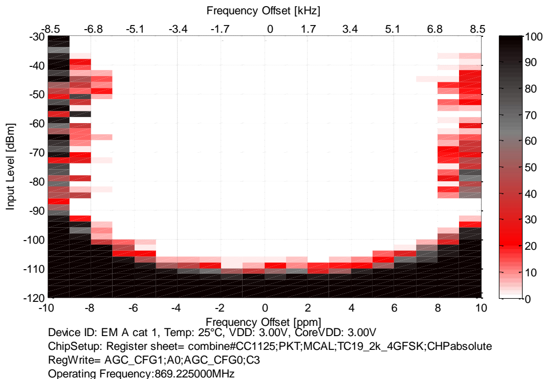
Figure 15. "Bathtub Plot". 19.2 kbit/s, 4GFSK, 25 kHz Filter Bandwidth
