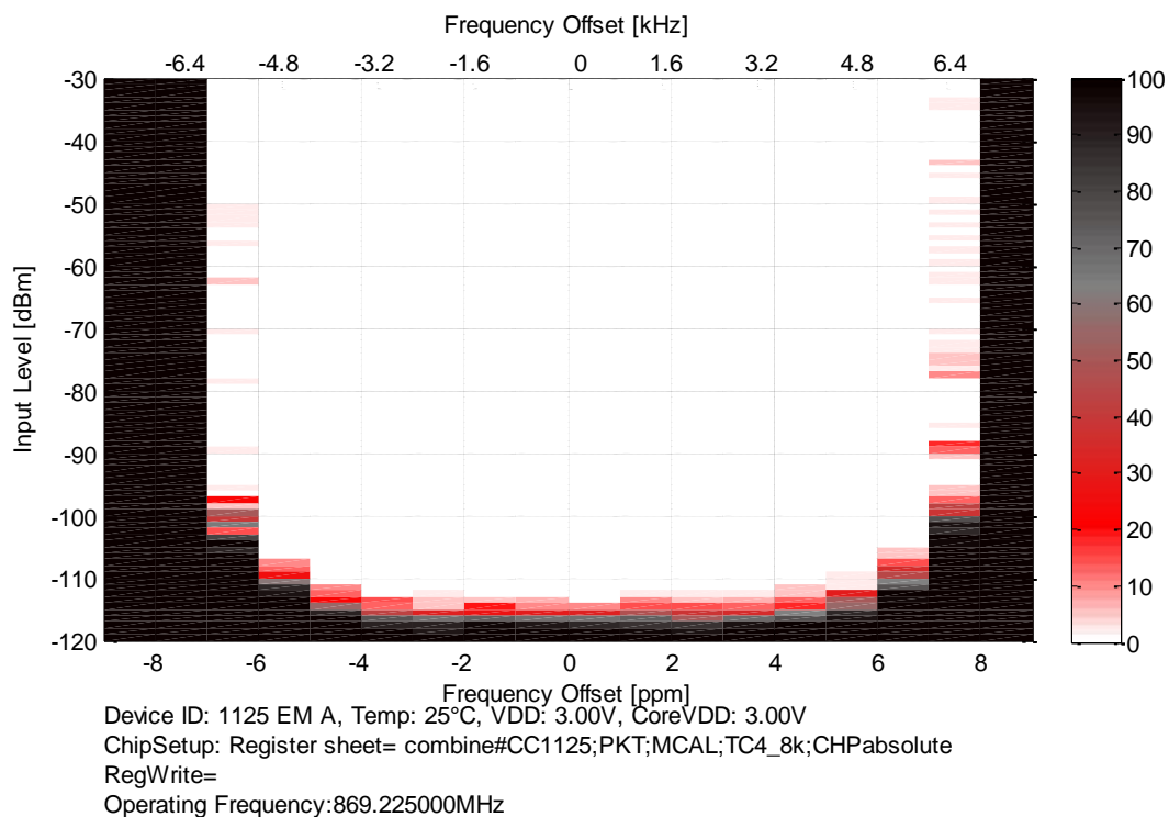
Figure 9. "Bathtub Plot". 4.8 kbit/s, ±2.4 kHz, 10 kHz Filter Bandwidth with FB2PLL
