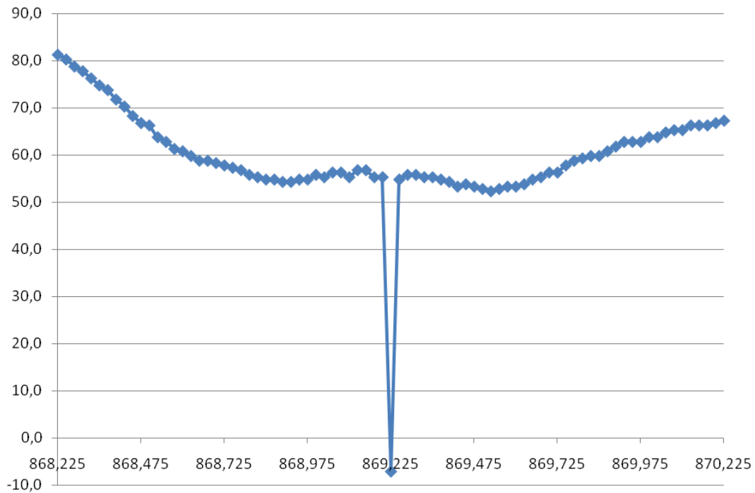
Figure 12. Spurious Response Rejection @4.8kbit/s, 16.6 kHz Filter Bandwidth with FB2PLL
