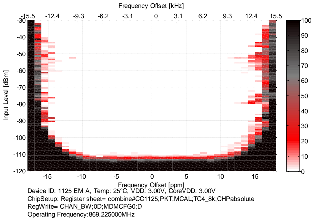
Figure 11. “Bathtub Plot”. 4.8 kbit/s, \pm 2.4 kHz, 19.2 kHz Filter Bandwidth with FB2PLL
