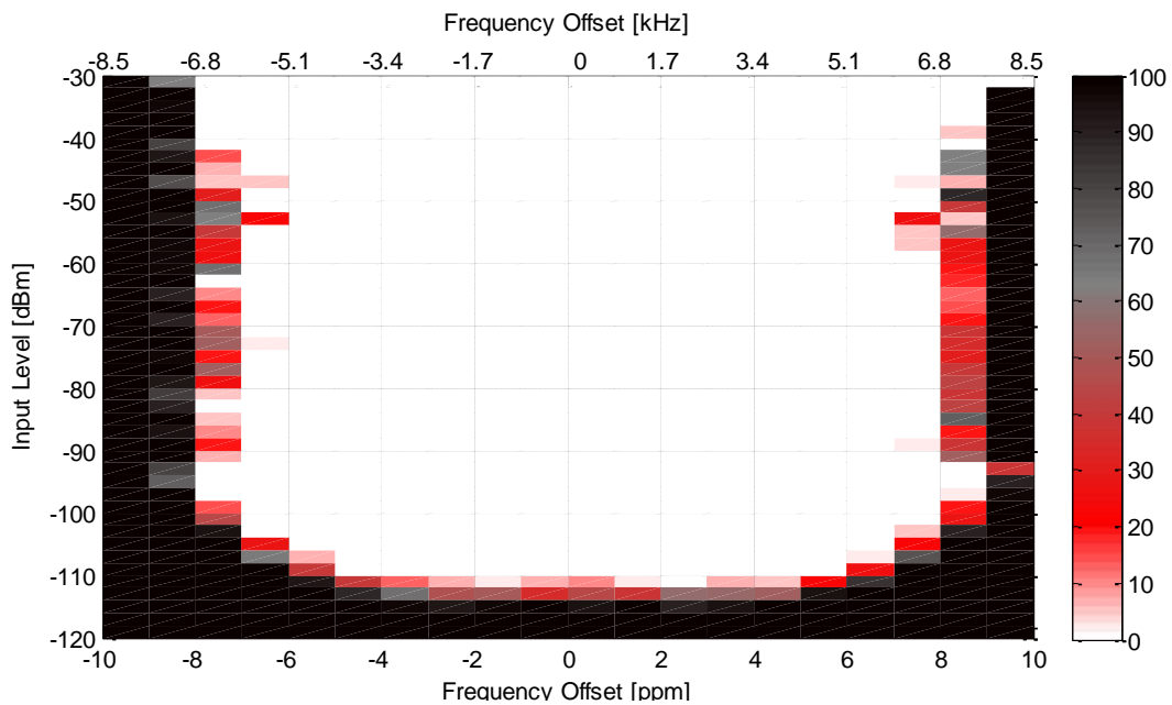
Figure 2. FB2PLL Disabled, 1 byte Preamble (4.8 kbit/s, 16.6 kHz Filter Bandwidth)
