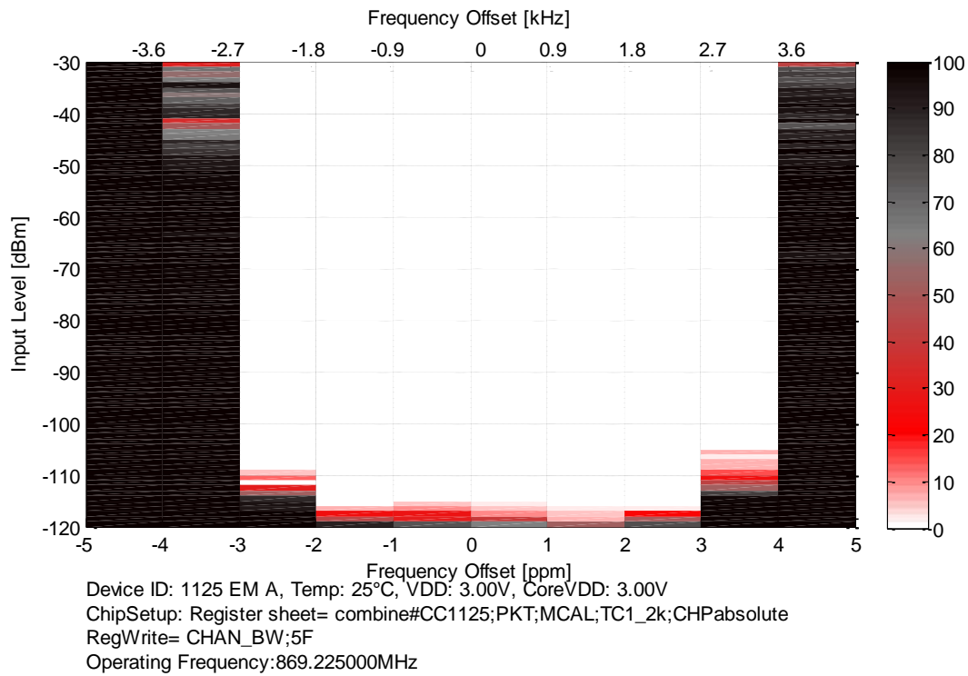
Figure 3. “Bathtub Plot”. 1.2 kbit/s, \pm 1.2 kHz, 5 kHz Filter Bandwidth with FB2PLL
