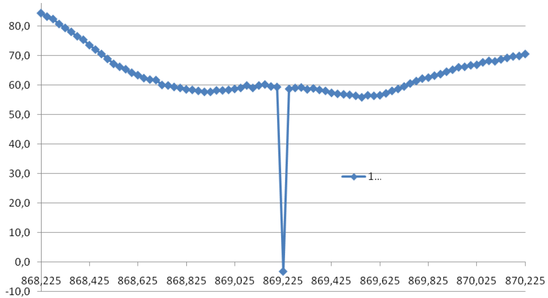
Figure 7. Spurious Response Rejection @1.2 kbit/s, 10 kHz Filter Bandwidth with FB2PLL
