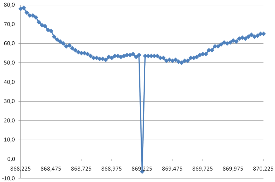
Figure 16. Spurious Response Rejection @19.2kbit/s, 25 kHz Filter Bandwidth
