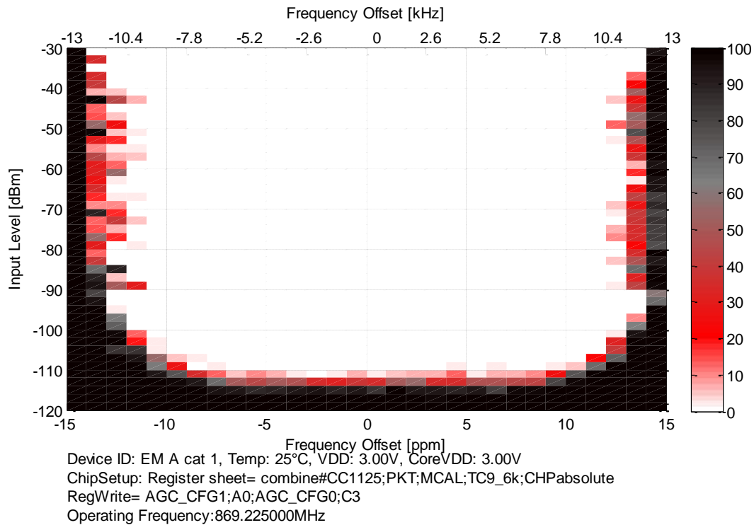
Figure 13. "Bathtub Plot". 9.6 kbit/s, \pm 4.8 kHz, 19.2 kHz Filter Bandwidth with FB2PLL
