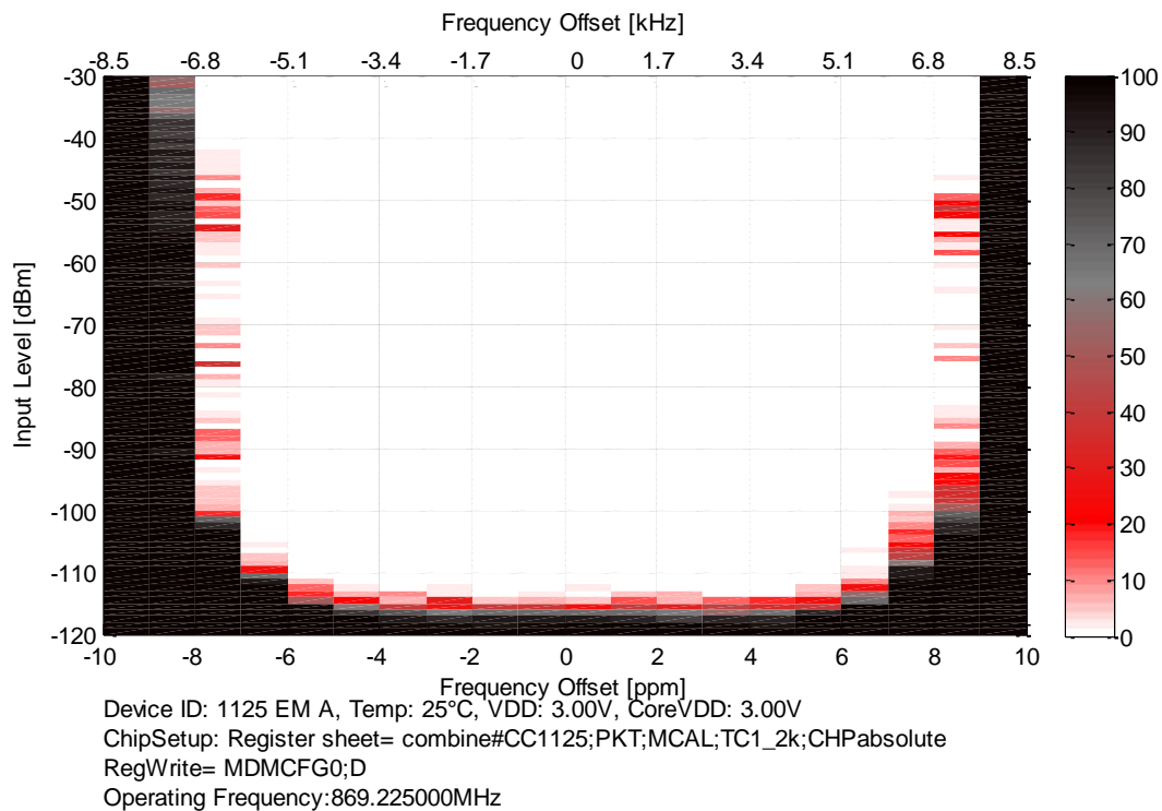
Figure 4. “Bathtub Plot”. 1.2 kbit/s, \pm 1.2 kHz, 10 kHz Filter Bandwidth with FB2PLL
