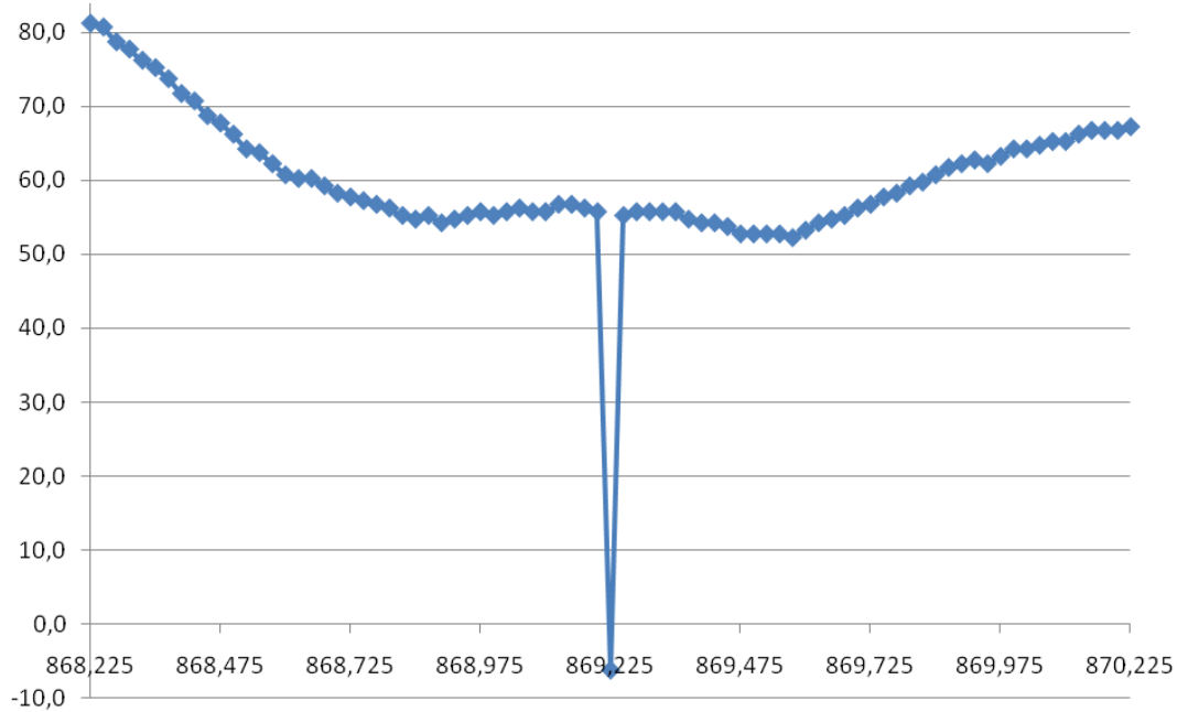
Figure 14. Spurious Response Rejection @9.6kbit/s, 19.2 kHz Filter Bandwidth with FB2PLL
