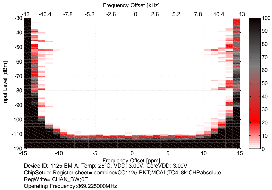
Figure 10. “Bathtub Plot”. 4.8 kbit/s, \pm 2.4 kHz, 16.6 kHz Filter Bandwidth with FB2PLL
